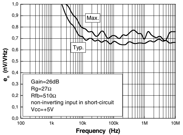
Figure 22. Input voltage noise (corner lot)
